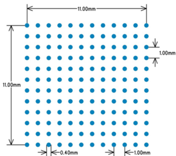
Figure 3: FBGA144 example land patterns (unit: mm)
