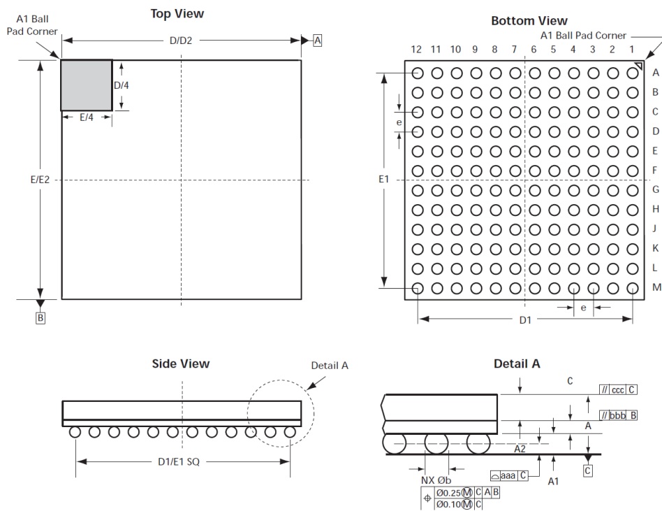
Figure 2: FBGA144 package outline drawings
