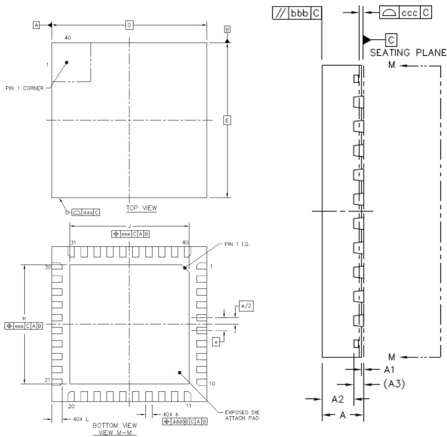
Figure 2: QFN40 6x6mm package outline drawings
