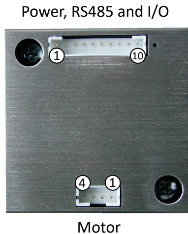
Figure 2: PD42-x-1370 connectors
