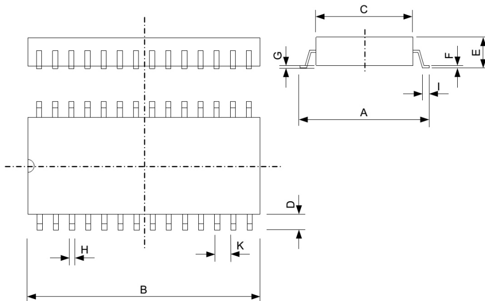
Figure 2: SO28 package outline drawings
