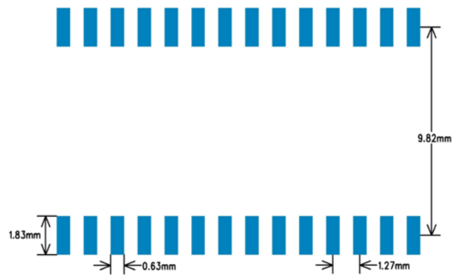
Figure 3: SO28 example land patterns (unit: mm)
