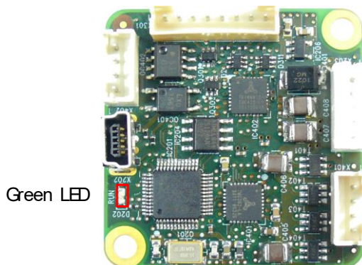
Figure 5.1 On-board LED
