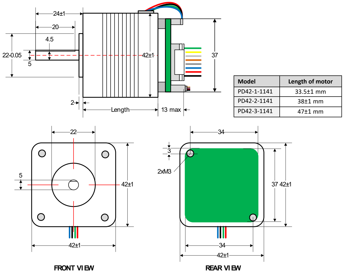
Figure 3.1 PD-1141 dimensions
