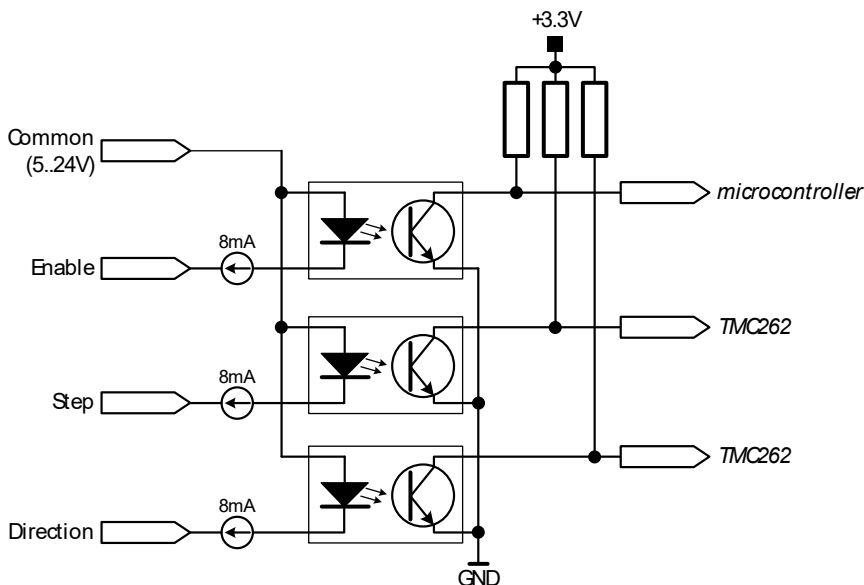
Figure 3.8 Step/Dir/Enable inputs
