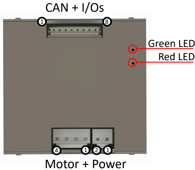
Figure 9: TMCM-1278 LED colors and loacation
