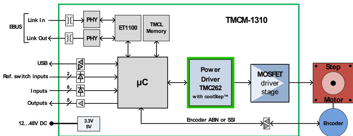
Figure 6.1 Main parts of TMCM-1310
