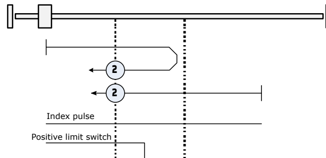
Figure 15: Homing Method 2
