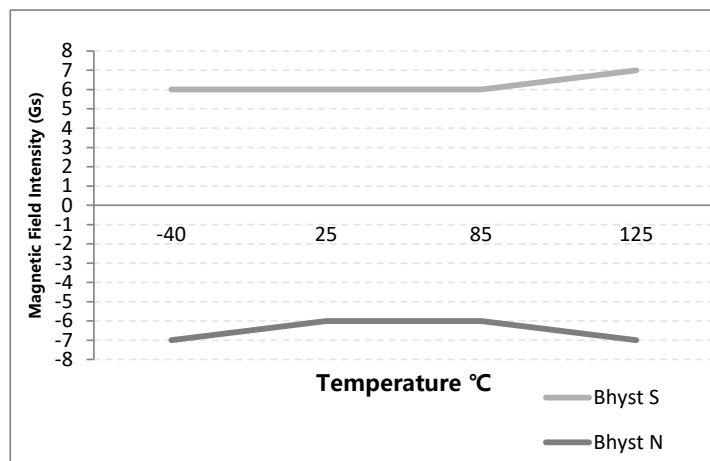
MT6325-L
