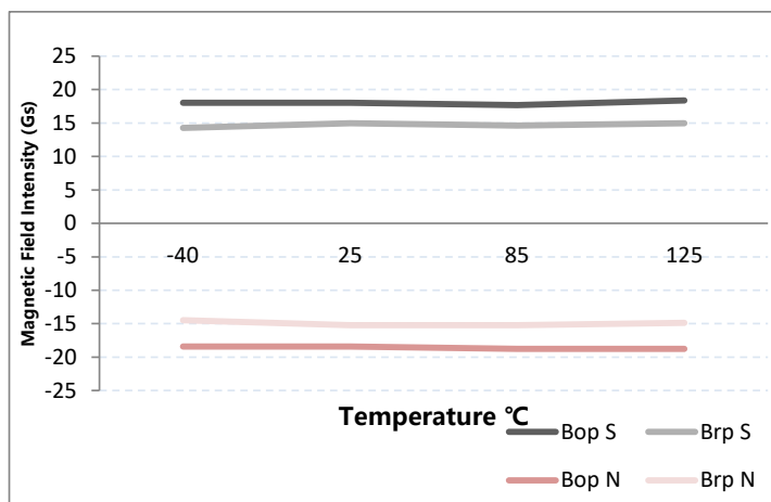
MT6325
