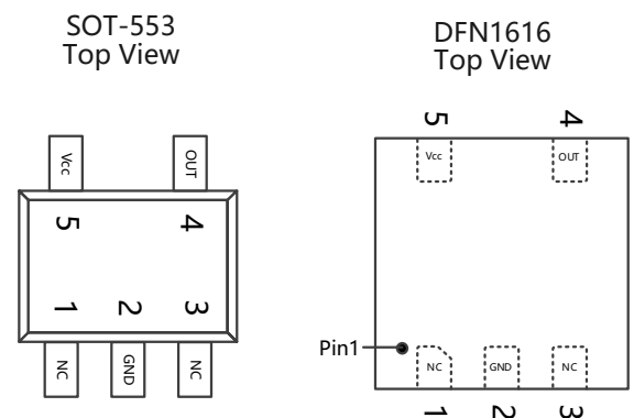
Figure.1 Pin Configuration & Functions
